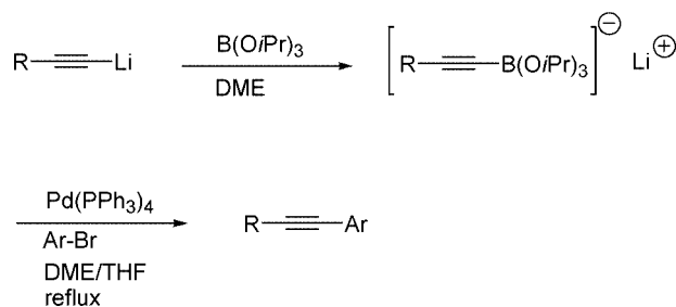
Scheme 1. Suzuki coupling of acetylenic boronic esters.
