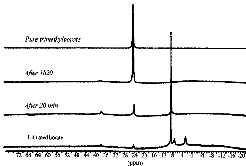
Figure 1. ^{11}\text{B} NMR signals during the Suzuki coupling of lithiated octynylboronate with p -bromotoluene.
