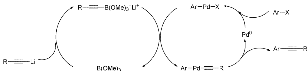
Scheme 3. \text{sp-sp}^2 Suzuki coupling reaction sub-stoichiometric in \text{B}(\text{OMe})_3 .
