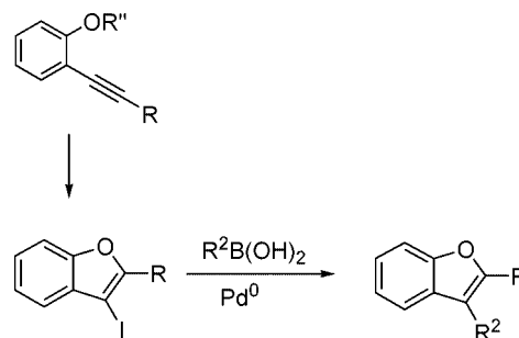
Scheme 2. Synthesis of 2,3-disubstituted benzo[ b ]furans.
